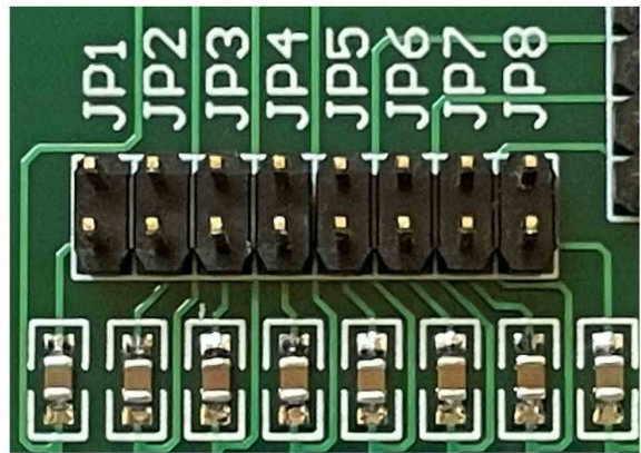
Figure 2 RFI Filter Jumper Location (shown without any jumpers enabled)
